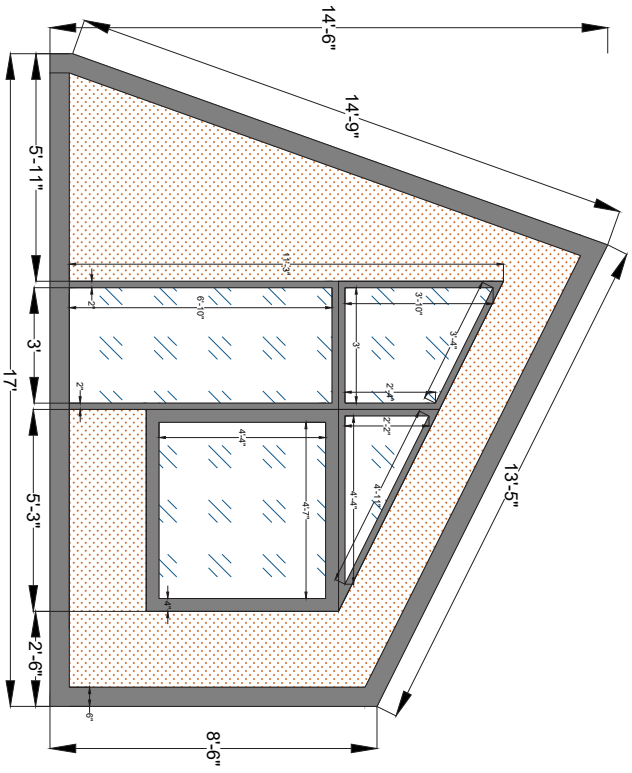
FRONT Elevation
